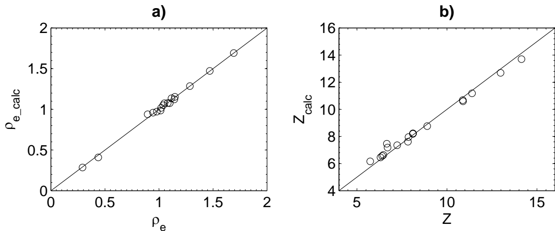
Figure 9-3.2: Calculated \rho_{e\_calc} and Z_{calc} versus the actual \rho_e and Z of 17 RMI materials (a, b).
